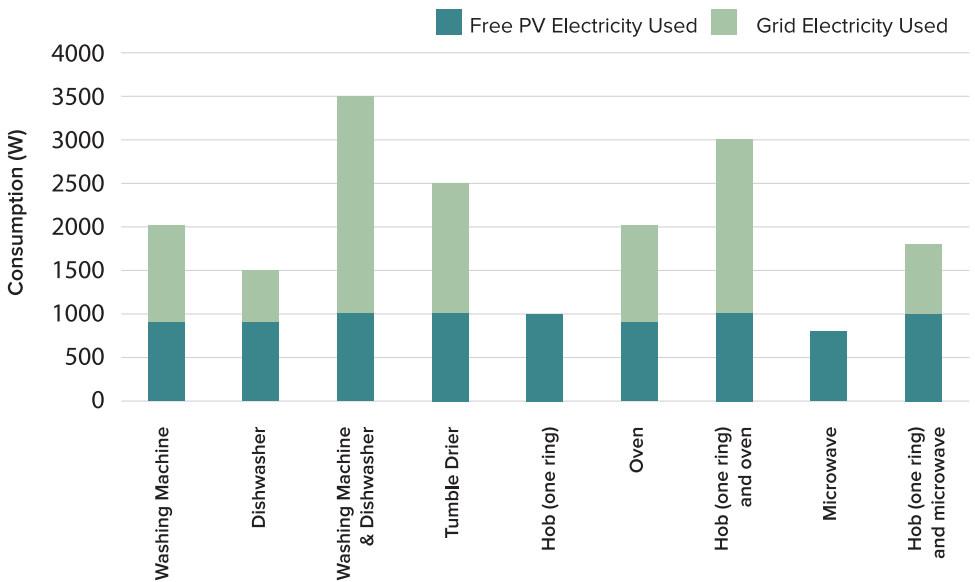
Figure 4 – Comparison of free solar PV and grid supplied electricity used by appliances for a solar PV system generating 1kW of electricity
